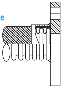
Raised Face Weldneck
