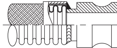
Male Part "A" Camlock
