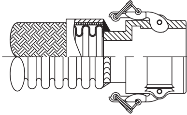
Female Part "D" Coupler
